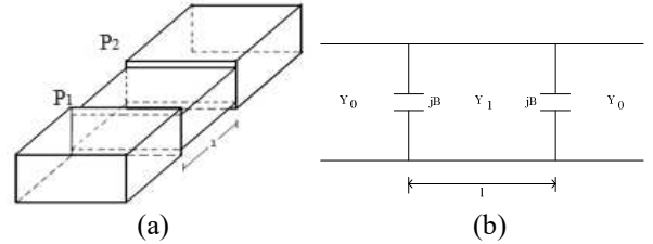
Figure 3. (a) Design model and (b) equivalent circuit of the mismatch waveguide section.
