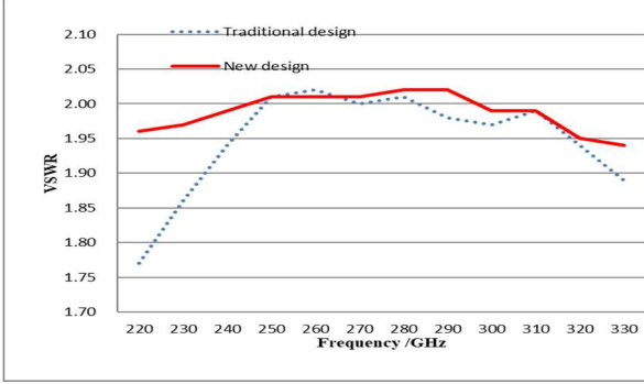
Figure 4. Simulation results of the mismatch waveguide with nominal VSWR 2.0 with different method (the dotted line is the traditional design, and the solid line is the new design)
