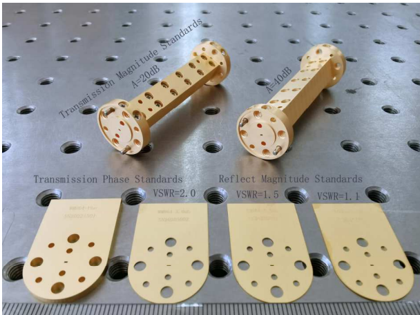
Figure 6. Photos of the processed verification standard.
