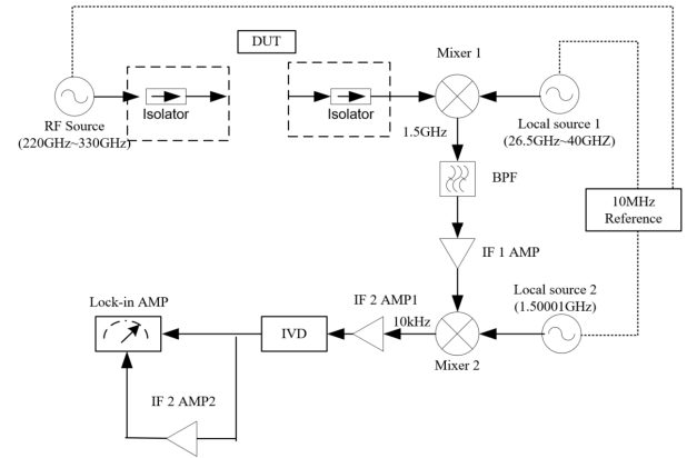
Figure 7. Block diagram of the attenuation measurement system
