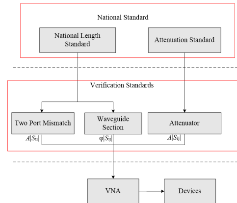
Figure 1. Traceability path of the 220GHz~330GHz S-parameter.
