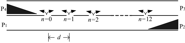
Figure 5. The internal structure of the attenuator.
