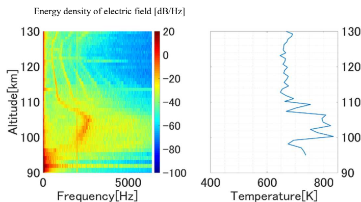
Figure 1. Altitude profile of electric field spectra and electron temperature during rocket ascent.
