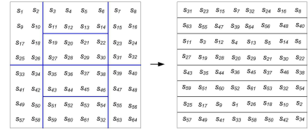
Original square matrix. Chaotic encrypted matrix.
