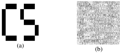
Fig.( 2) Watermark image. (a) Original watermark. (b) Chaotic encrypted watermark cr= 0.0181.
