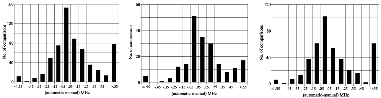
Fig 6. Differences between the values of f_oF2 scaled by the INGV software and by the standard manual method considering ionograms with a high level of radio noise. From the left to right the histograms show the result obtained for all the ionograms, daytime ionograms, nighttime ionograms respectively.
