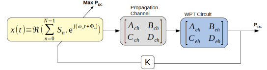
Figure 2. A WPT system seen as a closed loop. Propagation channel and rectifying circuit are modeled by their respective state-space models.
