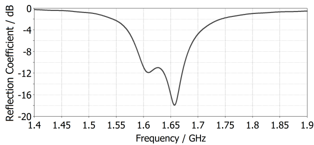
Figure 3. Simulated reflection coefficient.
