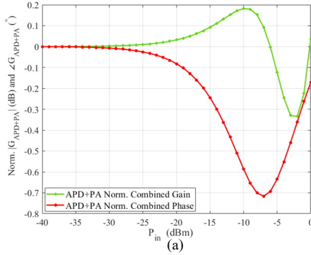
Figure 6. (a): Normalized APD+PA gain/phase variation with input power; (b): Predicted output spectrum for a 100 MHz signal at 1.9 GHz with an ideal PA (purple), with only the PA amplification (green), and with the APD+PA system (blue).
