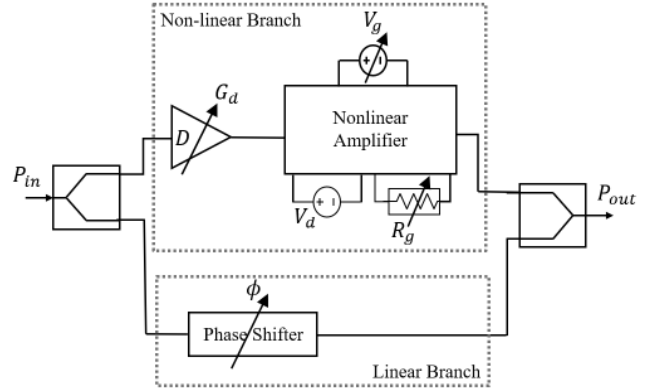
Figure 2. Architecture of the dual-branch APD linearizer used to correct the PA nonlinearities. The values of the driver gain, gate voltage, gate resistor of the amplifier, and phase shifter are optimized.
