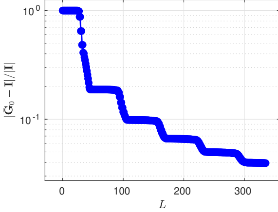
Figure 1. Convergence of the Gram matrix evaluated following our new semi-analytic approach (eq. (28)) to the expected value as a function of L .
