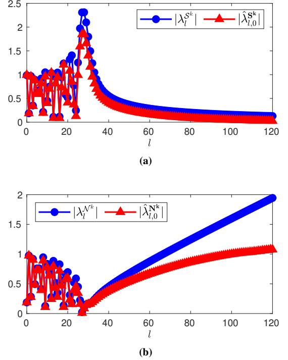
Figure 2. Eigenvalues of the BEM matrices of the single-layer (a) and hypersingular (b) operators: comparison with the spectra of the operators.
