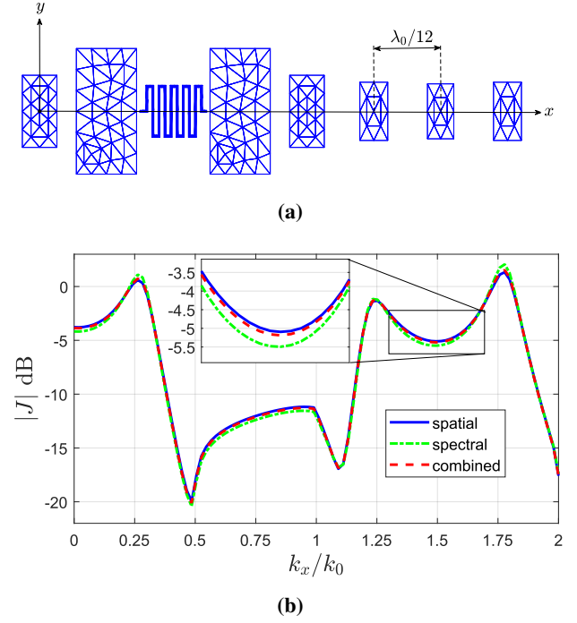
Figure 2. Simulation results for the array of 7 rectangular patches and 1 meander line. (a) Mesh. (b) Comparison of the simulated embedded element currents, for k_y = 0 .
