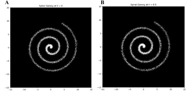
Fig. 1 Stereoscopic pair of spiral galaxies at time A) t=0 and B) t=0.5
