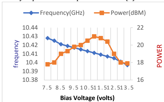
Figure 4: The results of the experiments indicate the bias tuning characteristics of the Gunn Oscillator that were used in the investigation (Gunn diode model no. MA49104-111 (25 mW))
