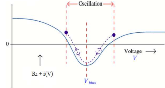
Figure3. Dynamic resistance of Gunn Diode
