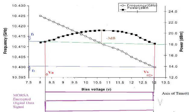
Figure:5 Marked frequency and space-frequency generation using a reflex klystron.
