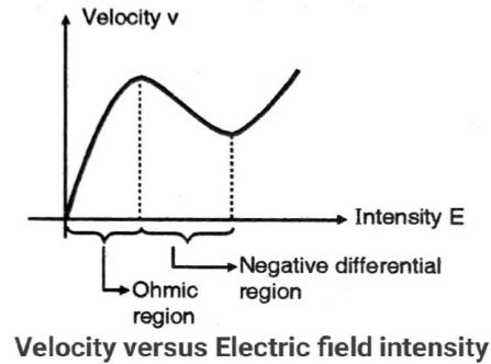
Figure 2. Microwave Gunn Characteristic
