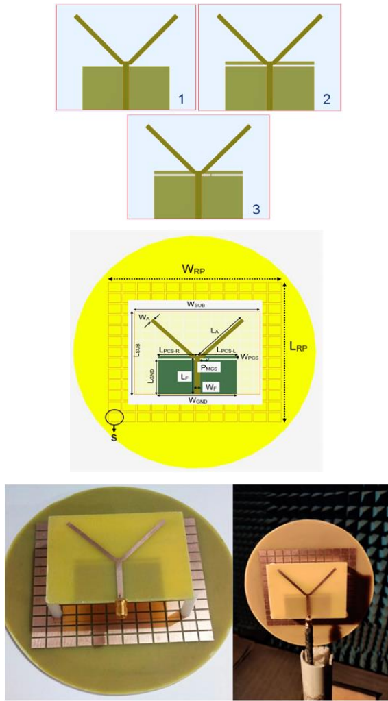
Figure 1. Proposed design: Schematic and Prototype with its placement in anechoic chamber for evaluating far-field.
