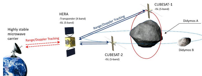
Figure 1. Concept of Hera Radio Science investigations. The figure highlights the main radiometric links between the various elements of the Hera mission that can be exploited to characterize Didymos gravity.
