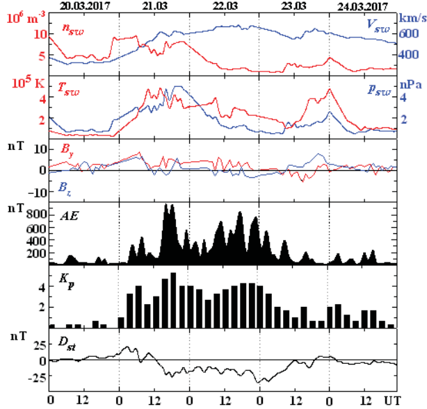
Figure 1. Variations of solar wind parameters: density n_{sw} , velocity V_{sw} , temperature T_{sw} and dynamic pressure p_{sw} ; IMF B_y and B_z components, AE , K_p and D_{st} indices.
