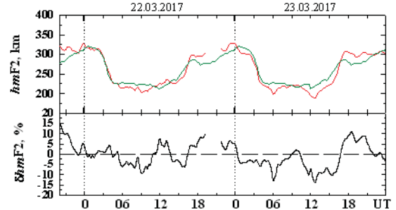
Figure 3. Temporal variations in hmF2 and \delta hmF2 .
