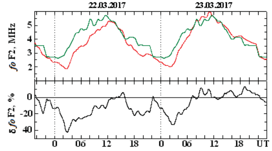
Figure 2. Temporal variations in foF2 and \delta foF2 .
