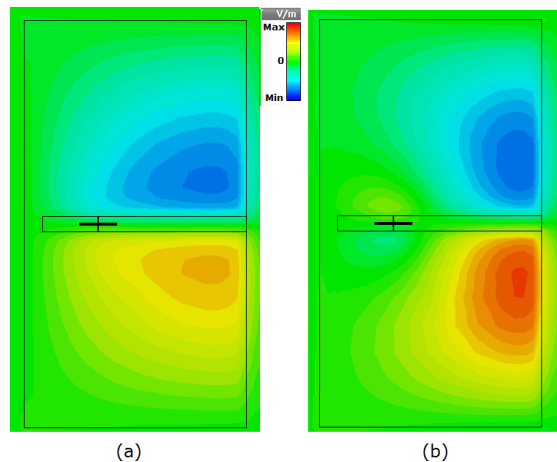
Figure 2. Z-directional E-field distribution inside the cavity at each resonance (a) 2.25 GHz (b) 3.42 GHz
