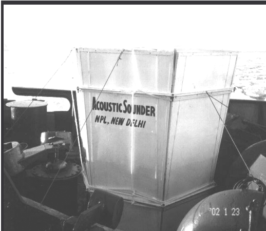
Fig.1. Shipborne acoustic sounder antenna mounted in the bow area
