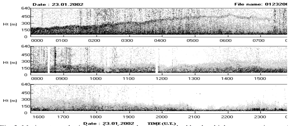
Fig. 3. Marine atmospheric boundary layer dynamics probed by the shipborne acoustic sounder reveals signatures of rising layer, a unique situation over the ocean-ice-air interface.
