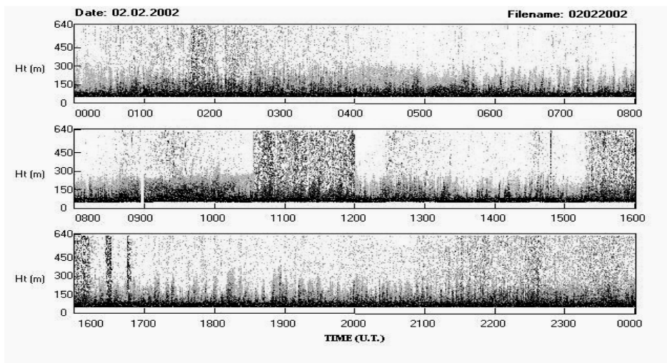
Fig. 4. Thermal convection over cold oceanic water reveals strong ocean-ice-air interaction.
