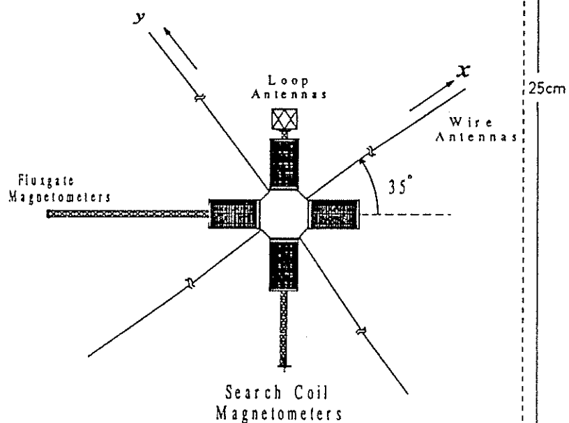
Fig. 1 VLF sensors on board the satellite
