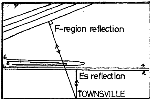
The small numbers in the Es layer indicate contours of equal plasma frequency (MHz). The tilt of the F-region is exaggerated for clarity but could be just a few degrees.
