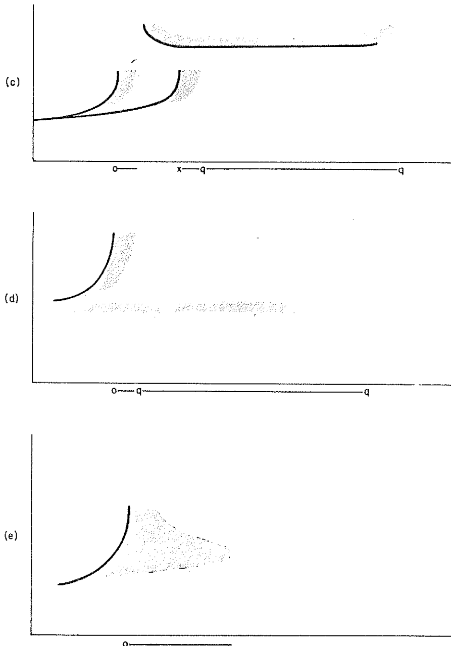
Fig. 6.10. f-plot convention when spread is present
