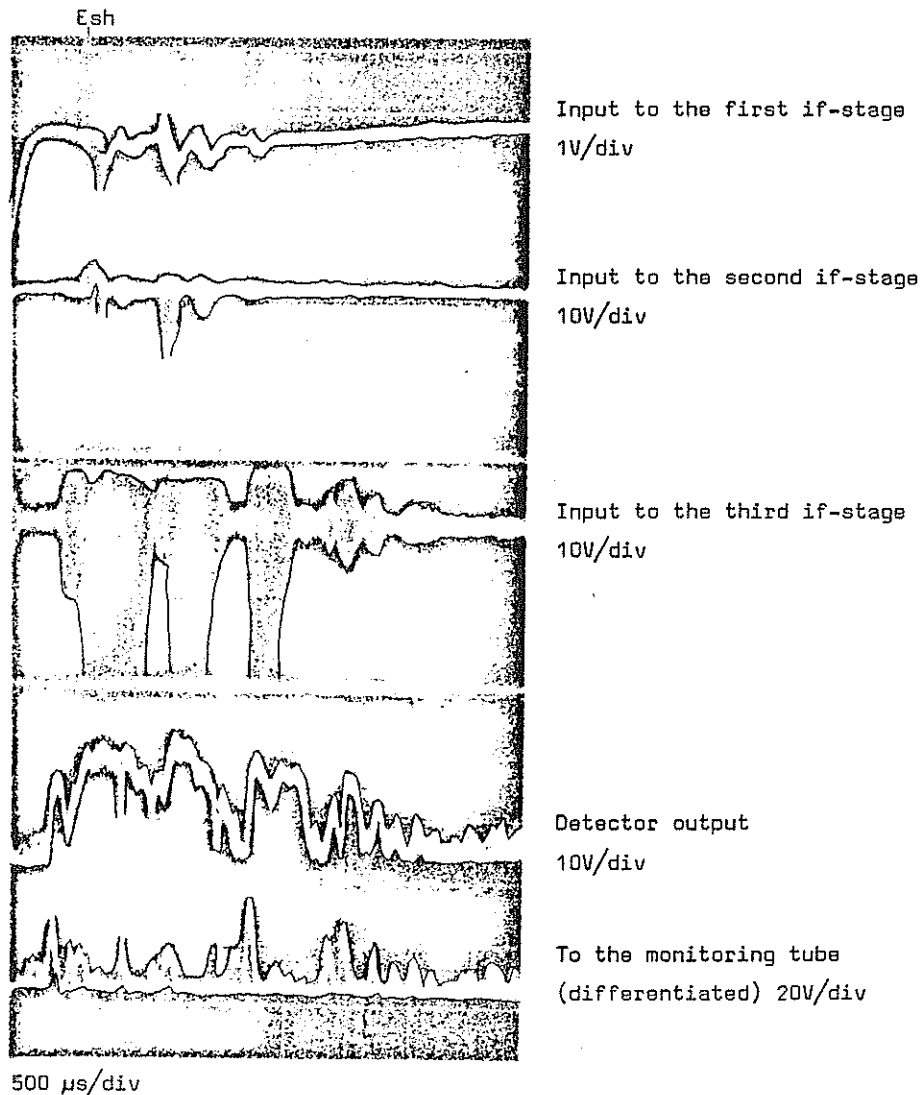
Fig. 3. Effects of too high gain and differentiation in ionospheric sounding. Ionosonde has 10 kW output power, pulse length 100 \mu s, antenna is rhombic, height of mast 64 meters. Frequency 2.7 MHz (0.25 MHz over foE). Ionosonde is located at Sodankylä.
