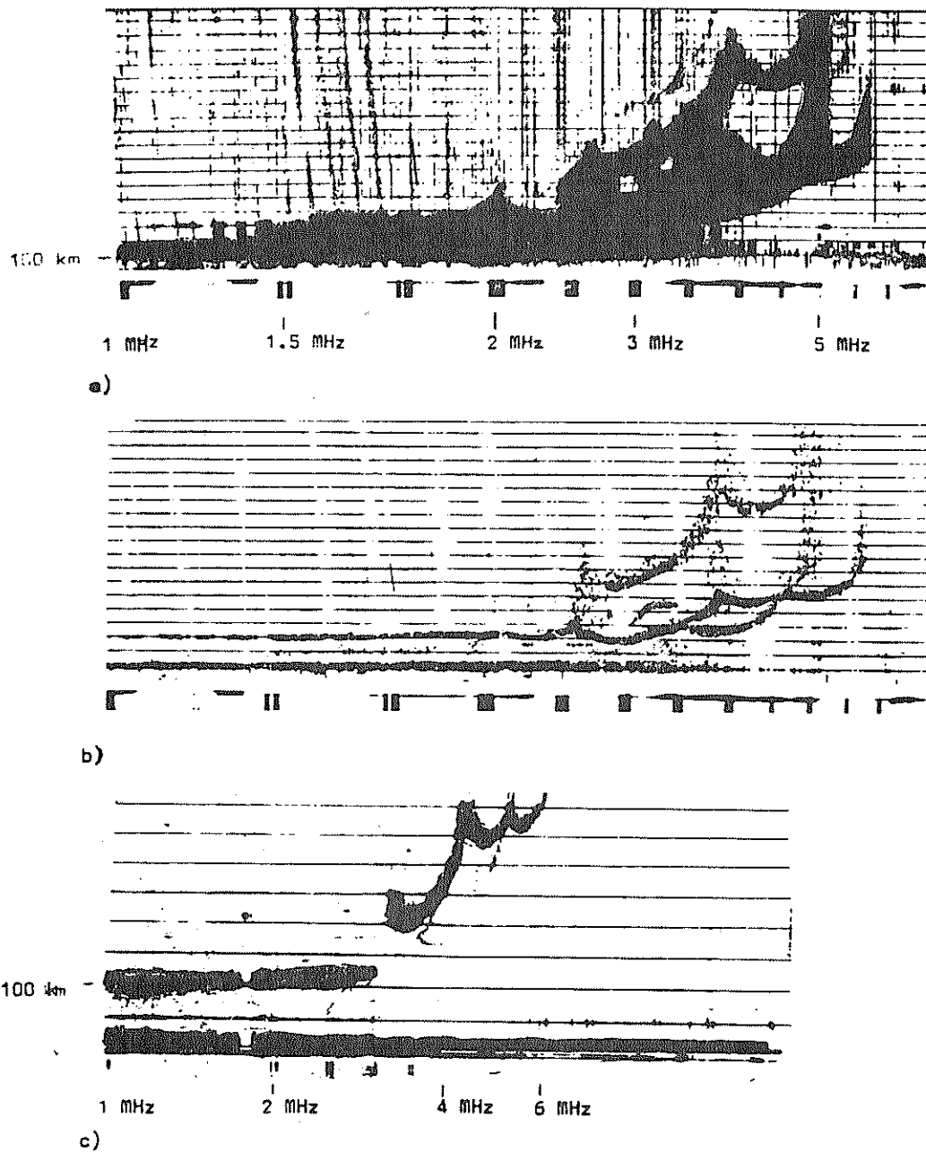
Fig. 2. a) High gain without differentiation b) High gain with differentiation, time constant approximately same as pulse length c) Low gain ionogram with differentiation, long time constant. Ionograms almost simultaneous 25.6.1973 13.40 LT, Sodankylä.
