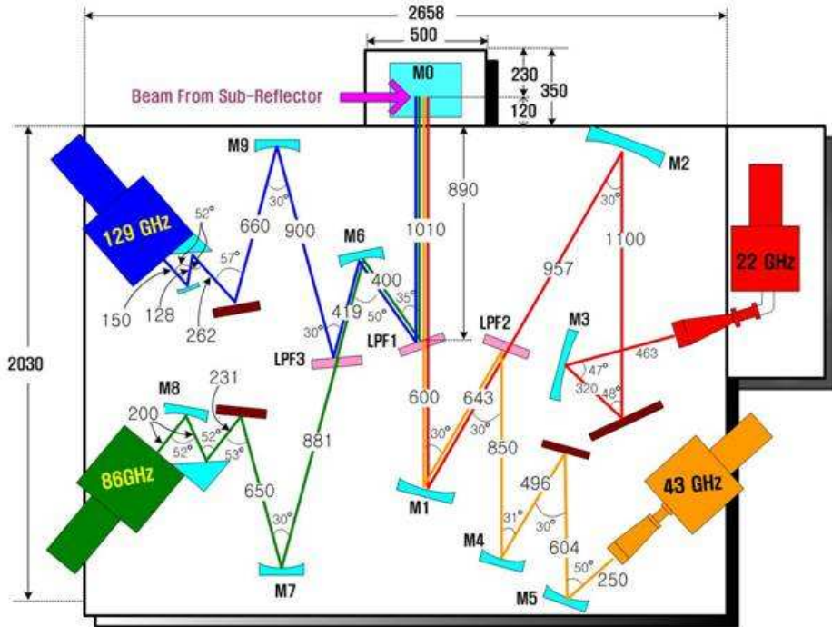
Figure 2: Quasi-optics system of KVN.
